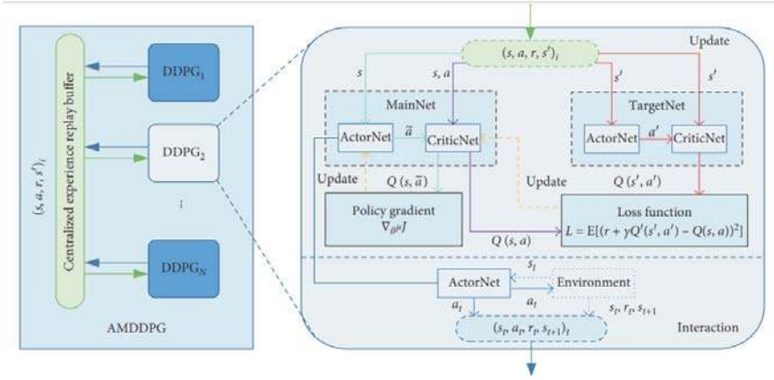
Figure 2. Structure of BAMDDPG.
