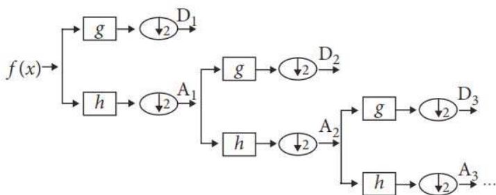
Figure 5. Wavelet transform.
