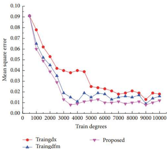
Figure 4. Convergence curve.
