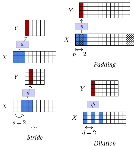
Figure 4.3: Beside its kernel size and number of input / output channels, a convolution admits three hyperparameters: the stride s (left) modulates the step size when going through the input tensor, the padding p (top right) specifies how many zero entries are added around the input tensor before processing it, and the dilation d (bottom right) parameterizes the index count between coefficients of the filter.
