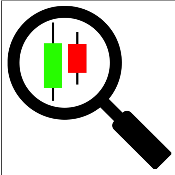
Inside Bar
