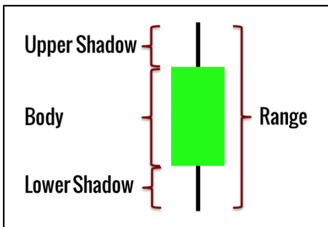
Beyond OHLC
