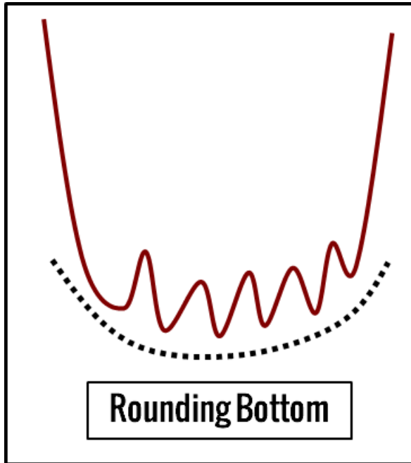
Rounding Bottom
