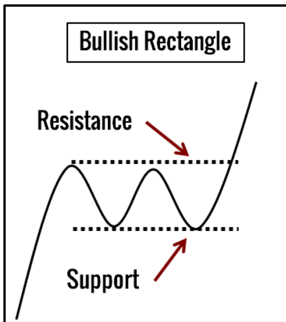
Bullish Rectangle
