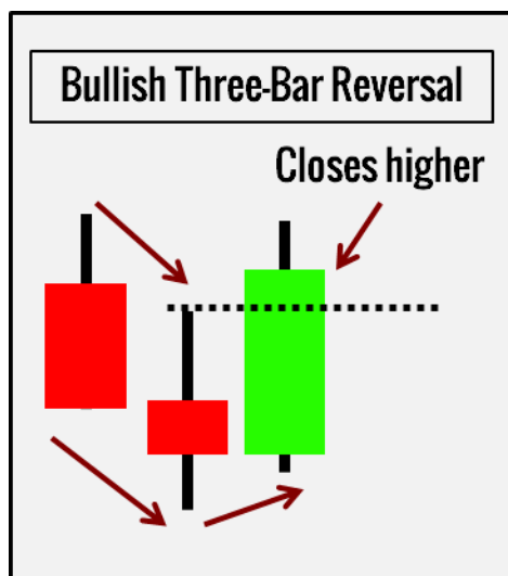
Three-Bar Reversal
