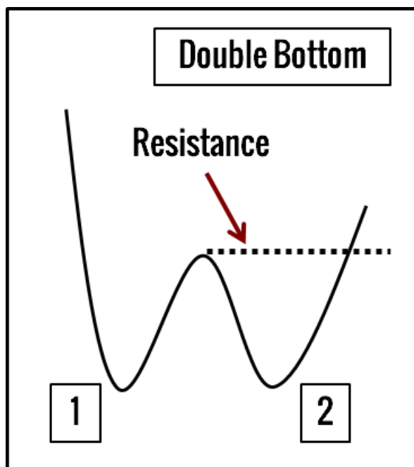
Double Bottom
