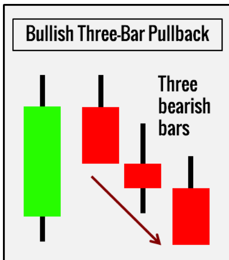
Three-Bar Pullback
