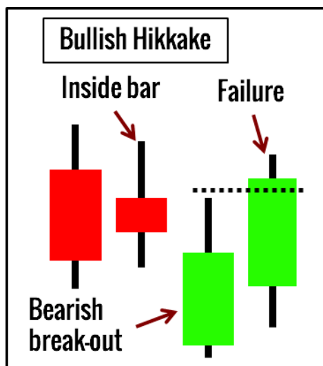
Hikkake Bullish
