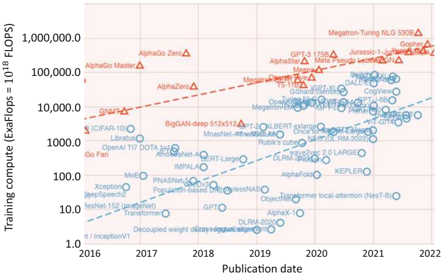
Fig. 8.3 Around 2016, a new trend of very large models emerged (red). These were developed by leading Internet companies that were able to finance the investment. The lower blue line illustrates the average computational effort of regular models, e.g. from universities. Note the logarithmic scale of the training compute. Image cutout from [76, p. 5]
