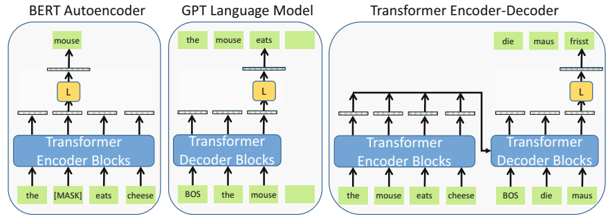
Fig. 2.16 Autoencoders like BERT (left) and autoregressive LMs like GPT-2 (middle) use transformer blocks to generate contextual embeddings of tokens. The transformer (right) combines a transformer encoder and an autoregressive transformer decoder to produce a translation. All models predict the probability of tokens with a logistic classifier L . Collectively these models are called Pre-trained Language Models (PLMs)
